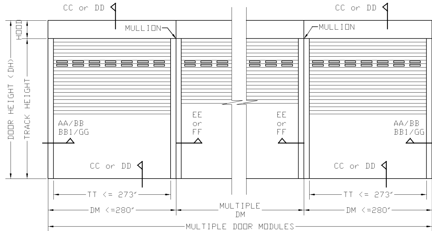
TYPICAL MULTIPLE UNITS ELEVATION
