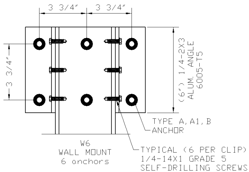
WALL MOUNT ANCHOR SELECTION
