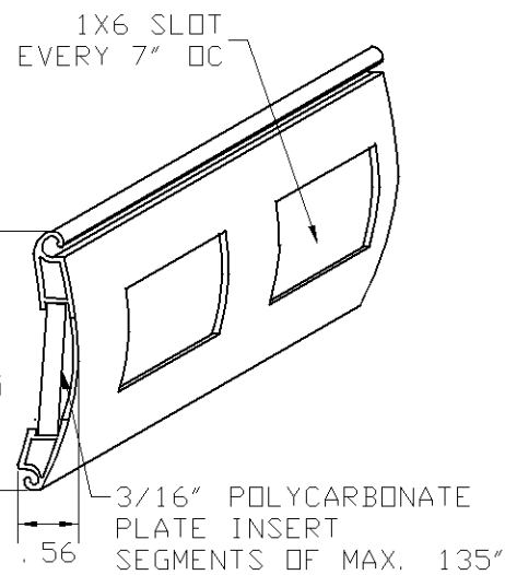
RE 1500VP WINDOW VIEW SLATS .05 EXTRUDED ALUMINUM 6063-T5 Alloy NOTE: MAXIMUM 2 SLATS PER DOOR
