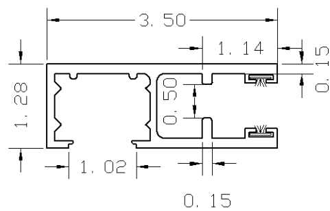
C- GUIDE RAIL W/ FELT 6005-T5 EXTRUDED ALUMINUM
