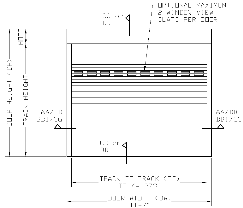
TYPICAL SINGLE UNIT ELEVATION
