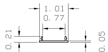
C1- TRACK SNAP COVER 6063-T5 EXTRUDED ALUMINUM
