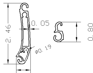
A- RE1500 ULTRA ER MALE & FEMALE SLATS 6063-T6 EXTRUDED ALUMINUM
